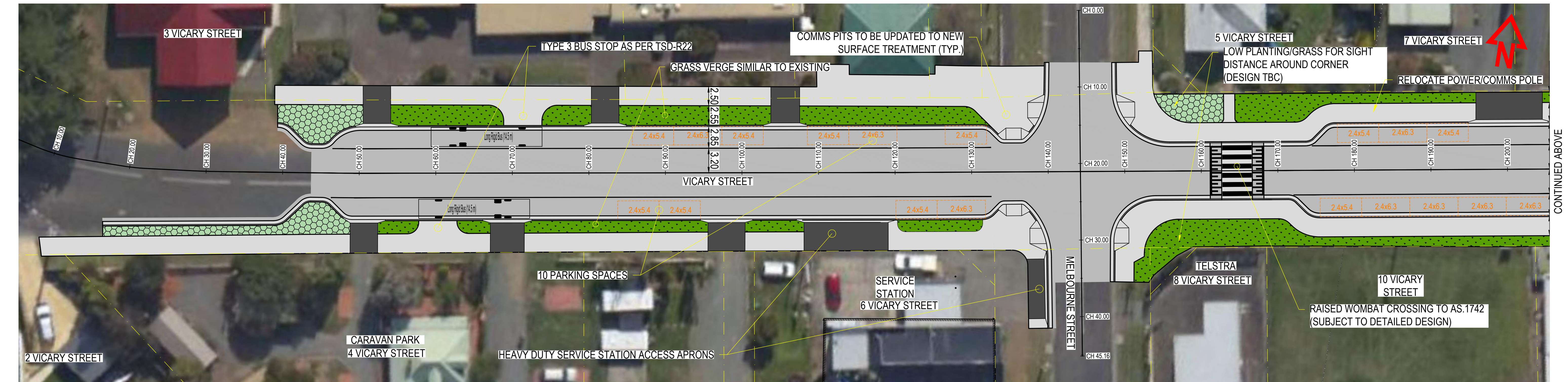
DETAIL SHEET VICARY SCALE 1:250
