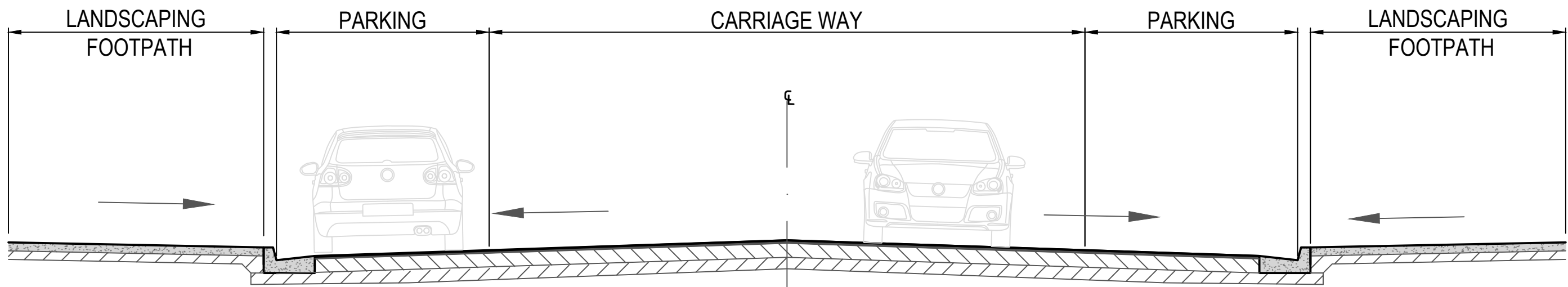
TYPICAL SECTION CHARLES & VICARY STREET SCALE 1:50
