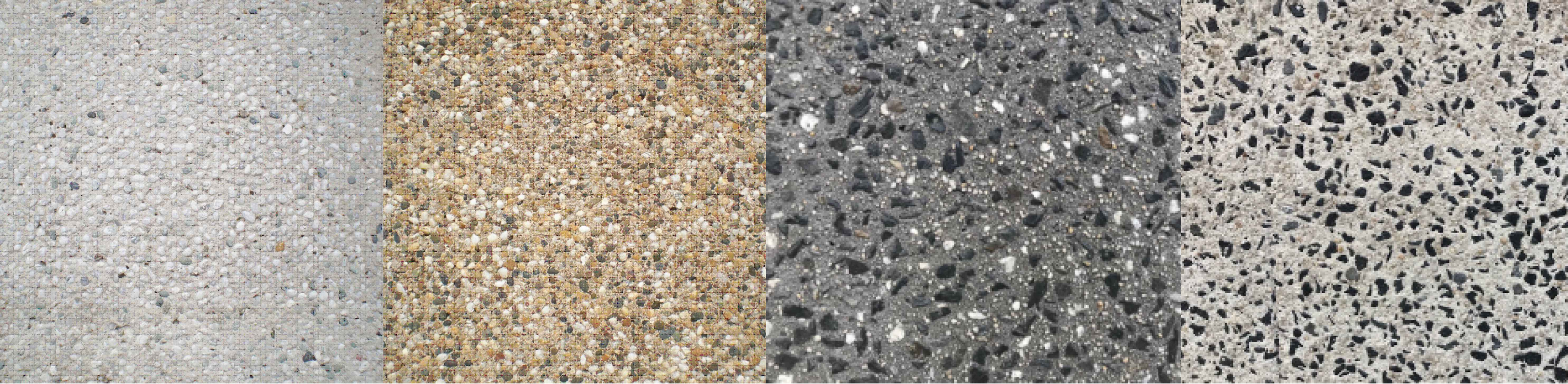
EXPOSED AGGREGATE CONCRETE FINISHES TO DELINEATE DIFFERENT ZONES
