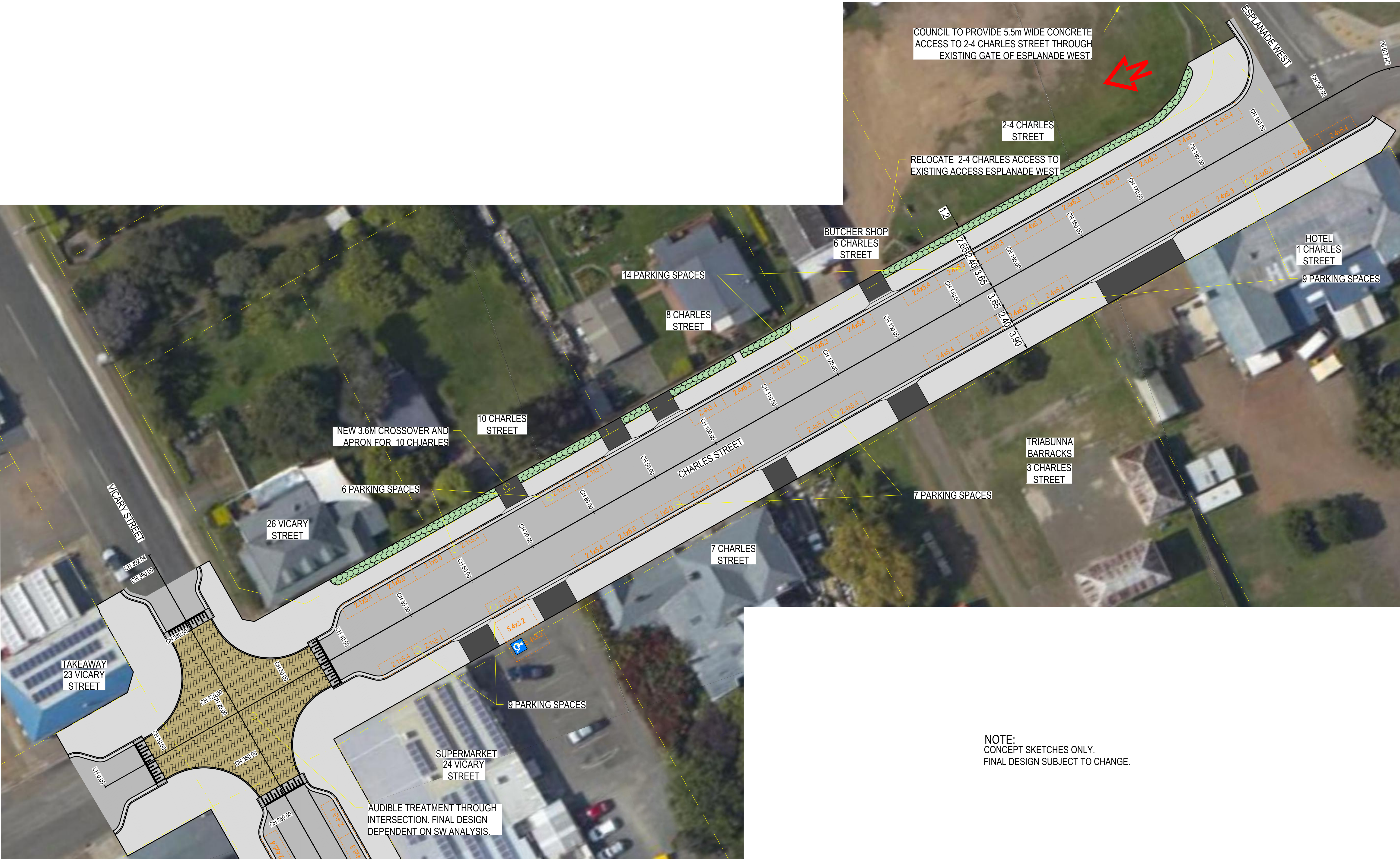
DETAIL SHEET CHARLES SCALE 1:250
