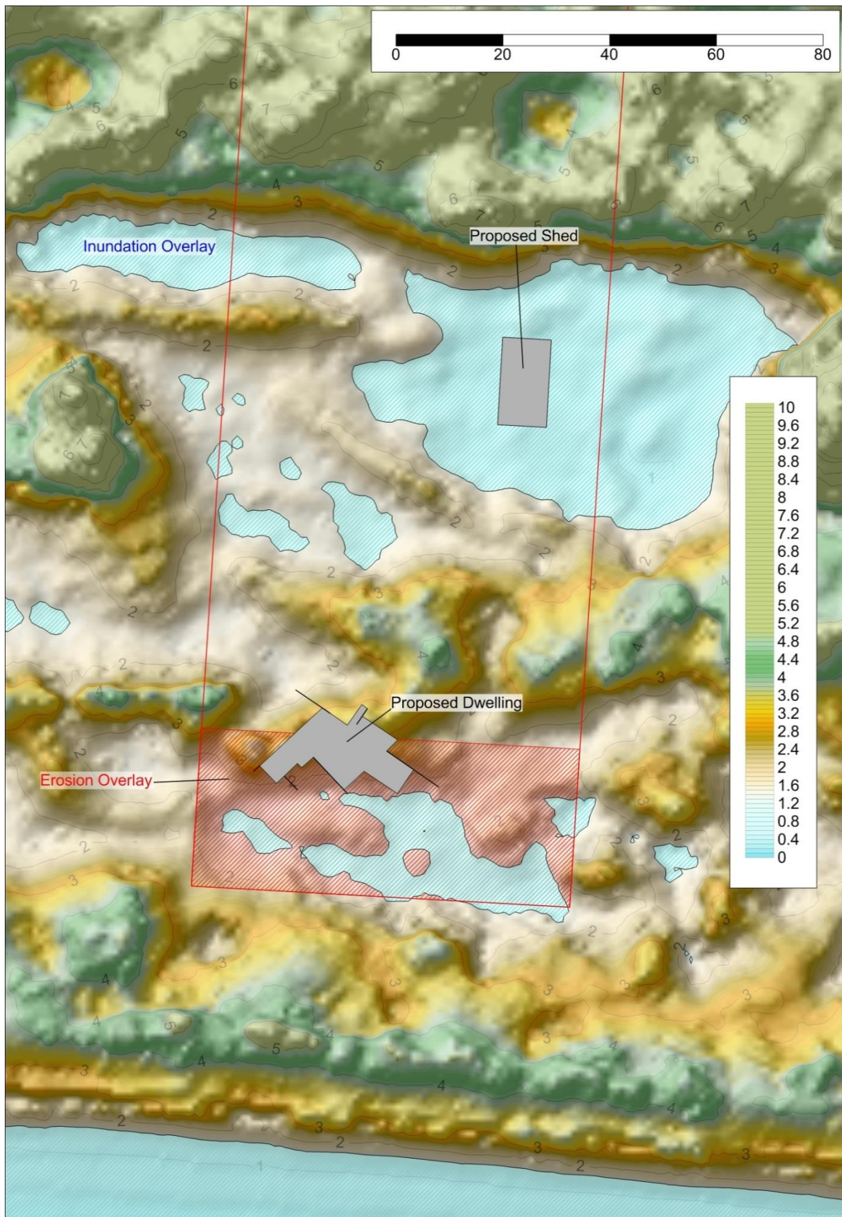
Figure 7 Site Geomorphology
