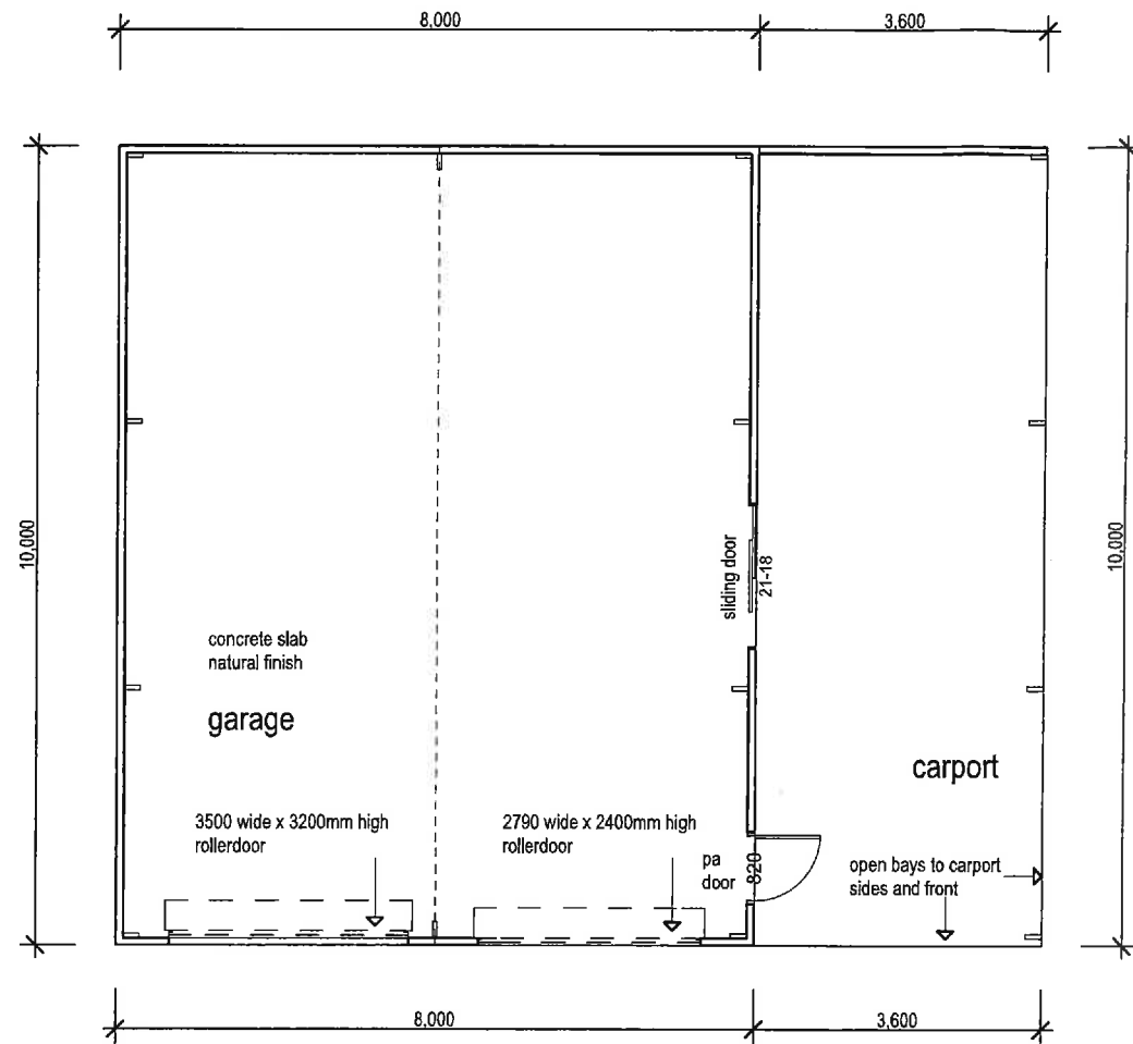
Floor plan
